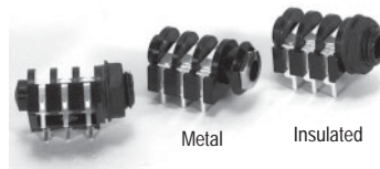
PCB mount
