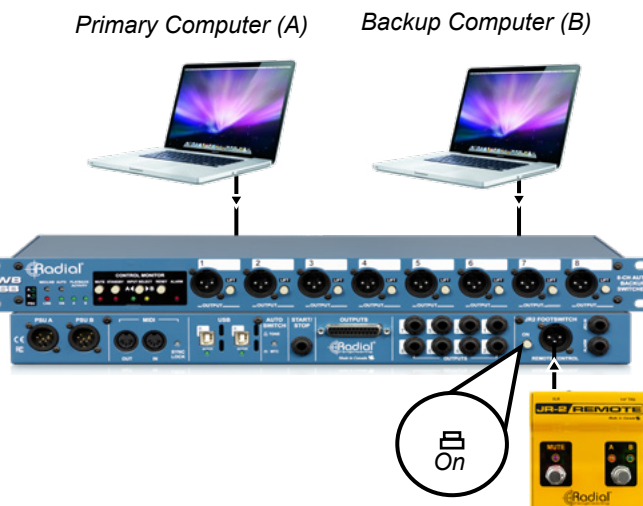
Manually switching to the backup computer using the JR-2 REMOTE footswitch
