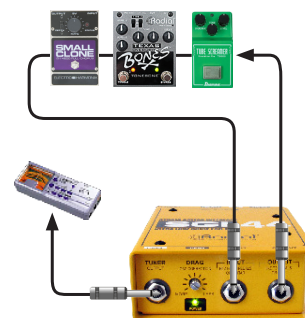
The 1/4" connections from the SGI-44 to a pedalboard.
