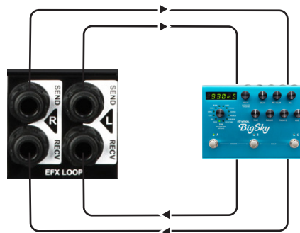
Connecting guitar pedals to the EFX Loop
