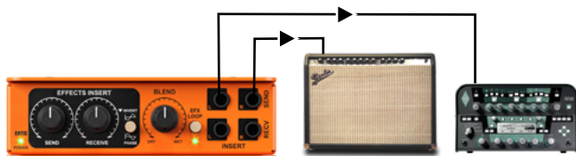
Connecting amplifiers and amp modelers to the EXTC Stereo
