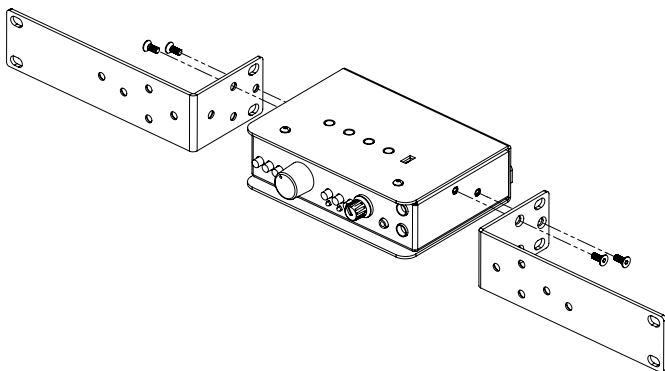
Double unit rackmounting
