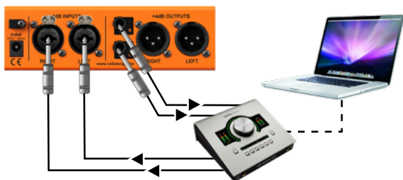
Connecting a recording interface to the EXTC Stereo using TRS cables
