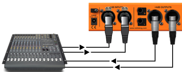
Connecting a mixer to the EXTC Stereo using XLR cables
