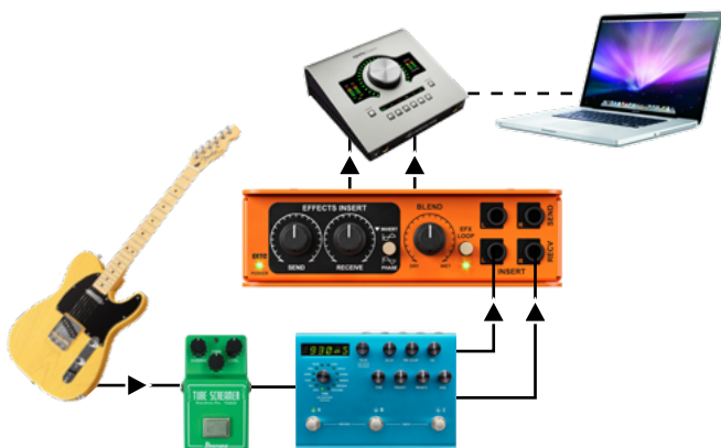
Using the EXTC Stereo for direct recording
