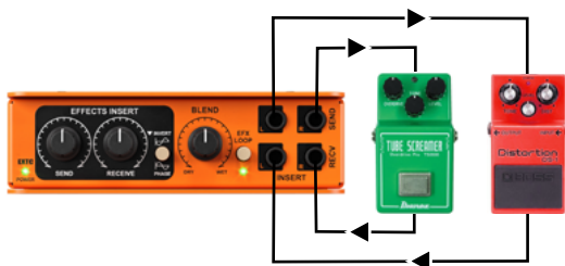
Connecting mono guitar pedals to the EXTC Stereo
