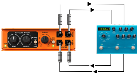
Connecting guitar pedals to the EXTC Stereo
