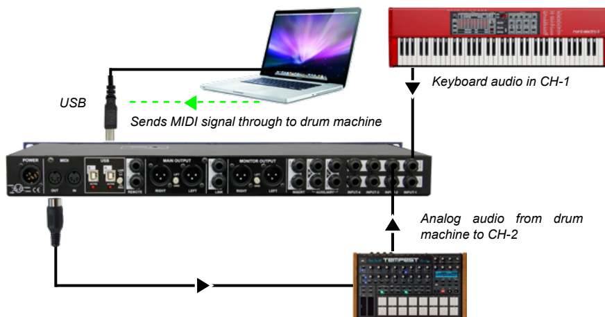
Using a laptop as the MIDI source to control an external drum machine
