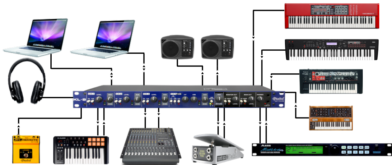
Utilizing the many connectivity options available on the KL-8
