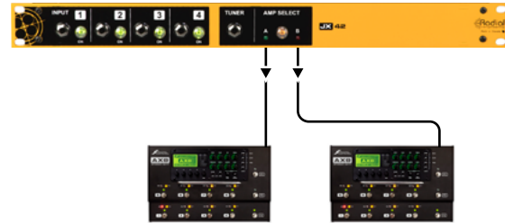
Connecting redundant amp modelers
